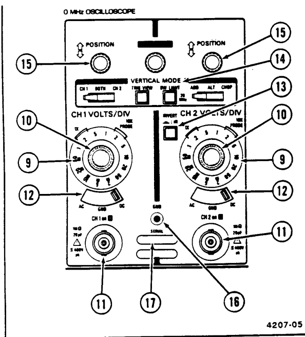
Figure 2-4. Vertical controls and connectors.
