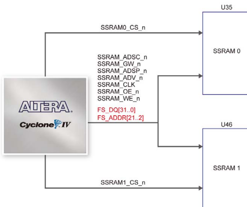
Figure 3-25 Connections between FPGA and SSRAM
