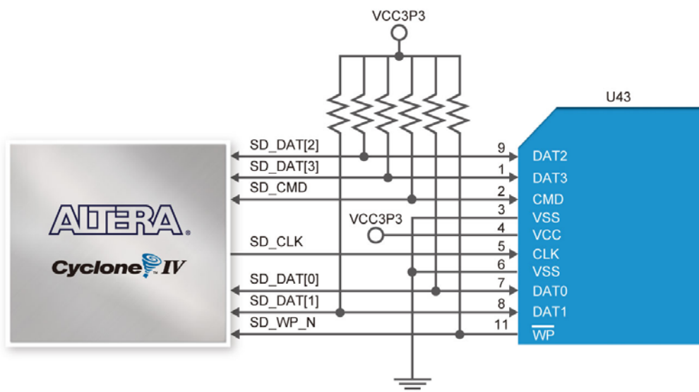
Figure 3-28 Connections between FPGA and SD Card Socket
