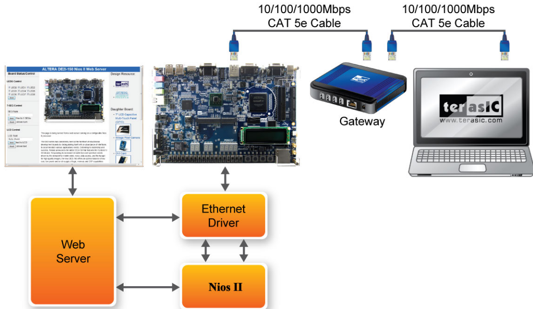
Figure 5-19 System Principle Diagram
