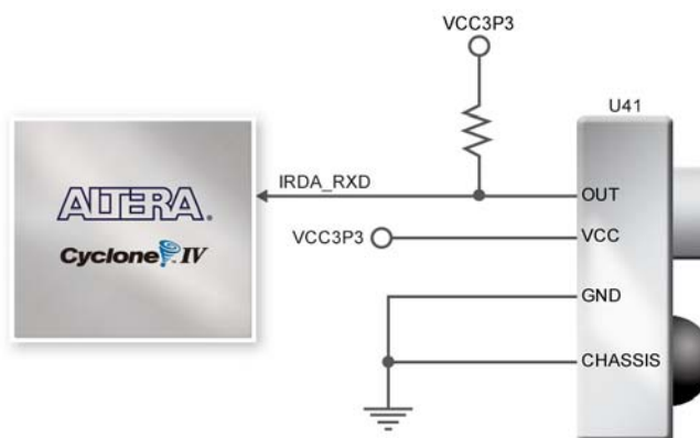
Figure 3-24 Connection between FPGA and IR
