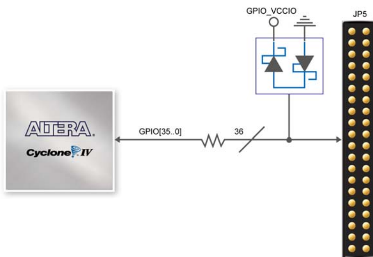
Figure 3-16 Connections between the GPIO connector and Cyclone IV GX FPGA
