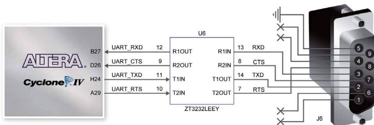
Figure 3-19 Connections between FPGA and ZT3232 (RS-232) chip
