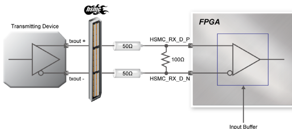
Figure 3-14 LVDS interface on HSMC connector and Cyclone IV GX FPGA
